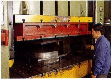
The blower casting is one piece, fabricated by a high performance hydraulic forming machine.
