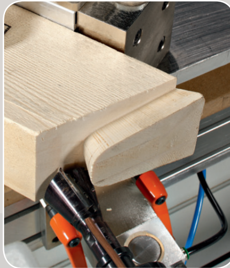
Head drilling/milling machining
